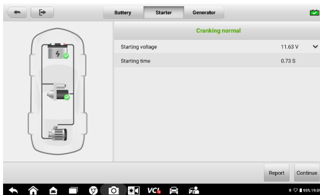
Figure 7-7 Starter Test Results Screen
